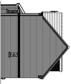
Side 1:200 scale
